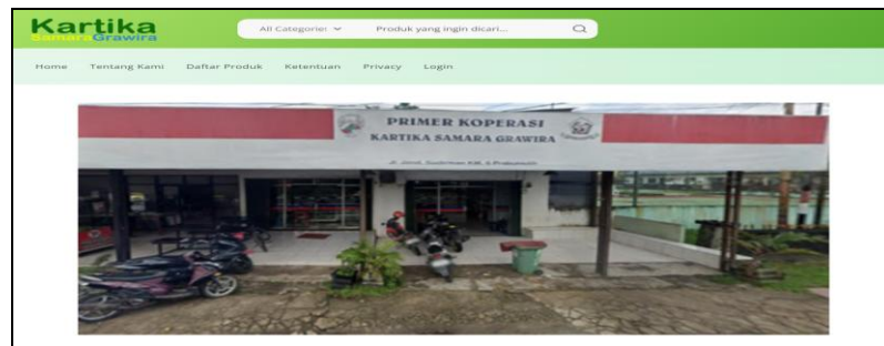
Gambar 7. Halaman Home
