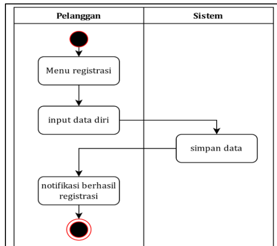
Gambar 2. Activity Diagram Registrasi
