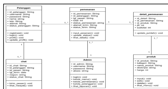
Gambar 6. Class Diagram
